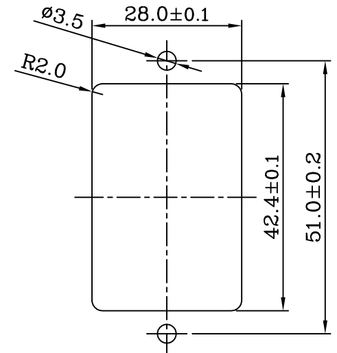
PANEL CUT-OUT
