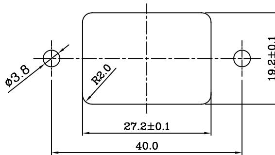
PANEL CUT-OUT
